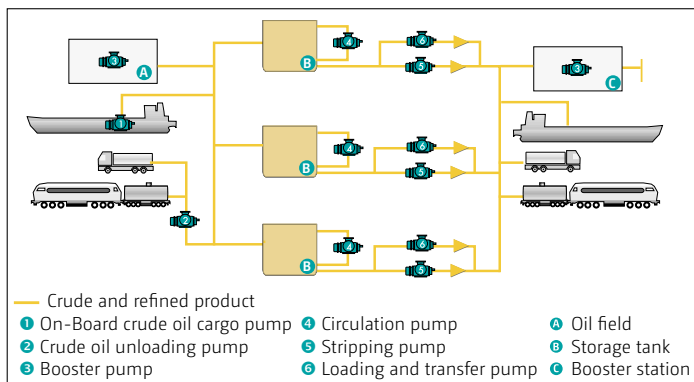
L4NC in tankfarm applications (illustration: Leistriz Pumpen GmbH)
